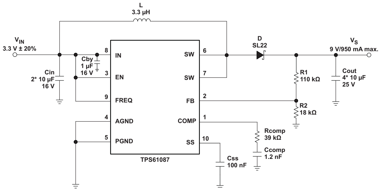
Figure 15. Typical Application, 3.3 V to 9 V ( f_s = 1.2\ \text{MHz} )
